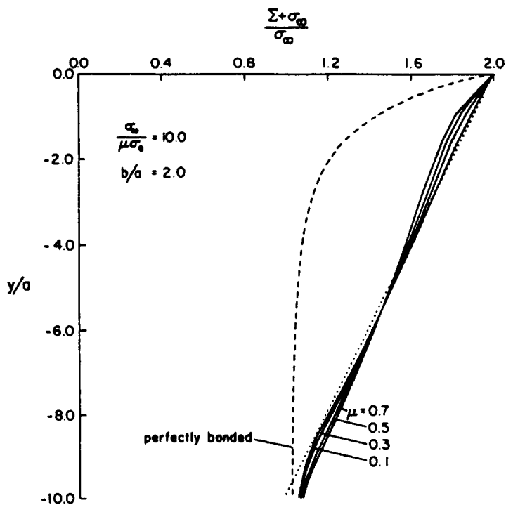
Fig. 12. Average fiber stress as a function of distance away from matrix crack. (—) Numerical solution to integral equation; (---) perfectly bonded interface; (- · -) constant shear stress approximation.
